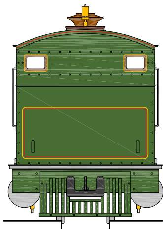
VICTORIAN RAILWAYS - NA 1 BALDWIN 10-20 1/4-D (1) - DRAWING 1 CONSTR. NO. 15936 - 1898 BALDWIN STYLE - LIGHT IVY GREEN & GOLD - STYLE 292
